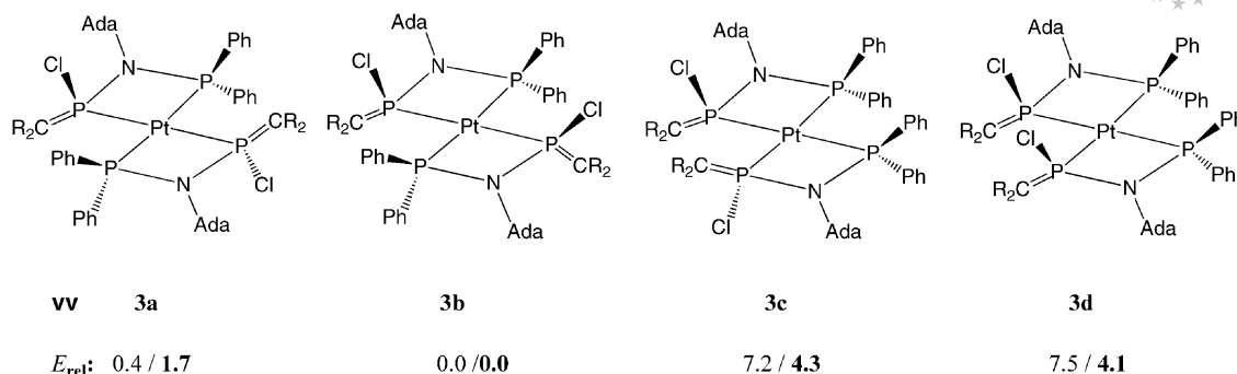
Scheme 2. Relative energies of complexes related to isomers 3a–3d ( R = \text{Me}_3\text{Si} ) for ligand 1' and for 1'' (in boldface) [(\text{H}_3\text{Si})_2\text{C}=\text{PN}(\text{Me})\text{-PR}'_2] , R' : Me ( 1' ), Ph ( 1'' )] in \text{kcal mol}^{-1} at the B3LYP/B//B3LYP/A level of theory (see ref. [15] ).
