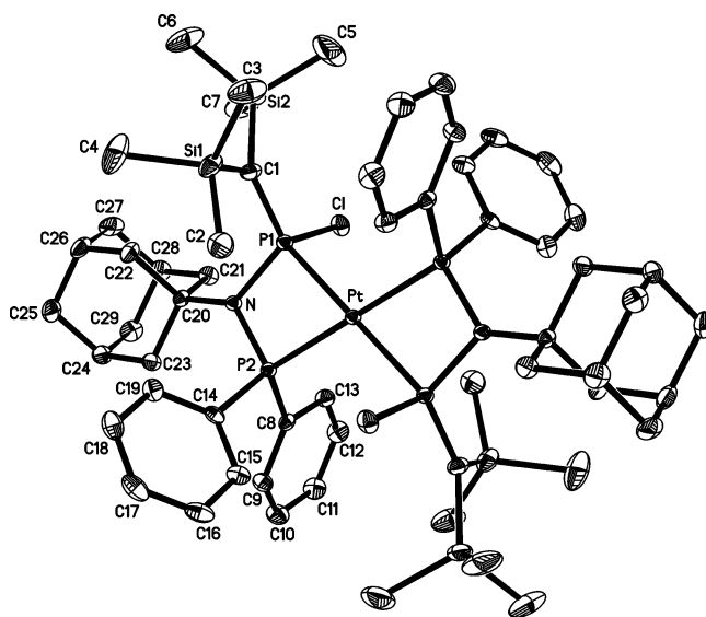
Figure 1. Molecular structure of 3a . Selected bond lengths (Å) and angles (°): P1–Pt 2.3411(5), P2–Pt 2.2900(5), P1–C1 1.673(2), P1–N 1.7617(17), P2–N 1.6945(16), P1–Cl 2.1107(7), P1–N–P2 100.96(9). Hydrogen atoms are omitted for clarity. Atoms are drawn as 50% thermal ellipsoids.
