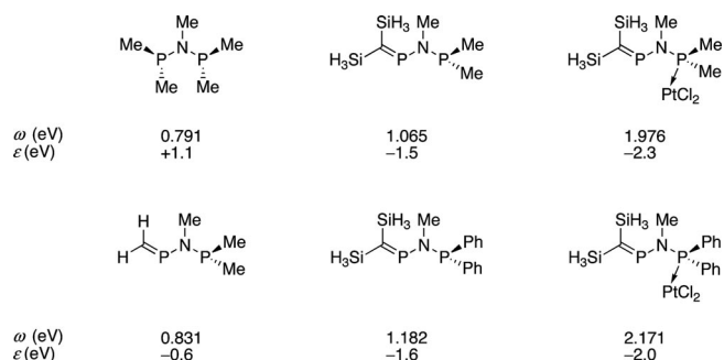
Scheme 3. Electrophilicity indices ( \omega , in eV, B3LYP/6-311+G**//B3LYP/6-31+G*[15b]) and the \pi^*_{C=P} Kohn–Sham orbital energies ( \epsilon , in eV, B3LYP/6-31G**/B3LYP/6-31+G*) for various PNP model compounds.
