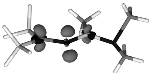
Figure 2. Representation of the Fukui function for nucleophilic attack [f^*(r)] in the case of (H_3Si)_2C=PN(Me)PMe_2 calculated at the (U)B3LYP/6-311+G**//B3LYP/6-31+G* level of theory.
